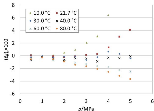
Figure 9. Relative deviations of f(T, p) data to the calculated values, (\Delta f)_r , where the calculations use values of B_{12} from Ref. 6 and assume C_{112} = C_{122} = 0 .
